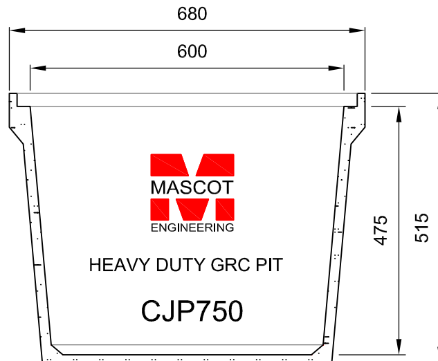
SECTION VIEW
